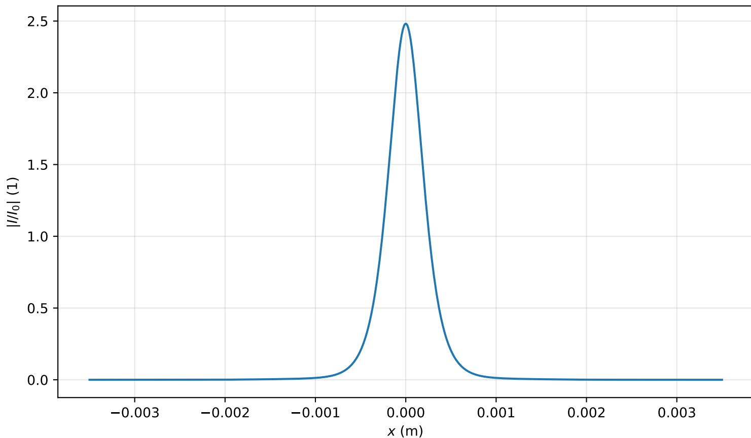
Intensity profile I(x, y = 0, z = 2.707m)/I_0 , P_{in}=1.0P_{cr} , artificial time
